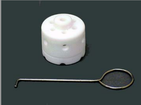
#8768E 10mm Square HF Compatible Chip Holder with Chip Holder Handle
