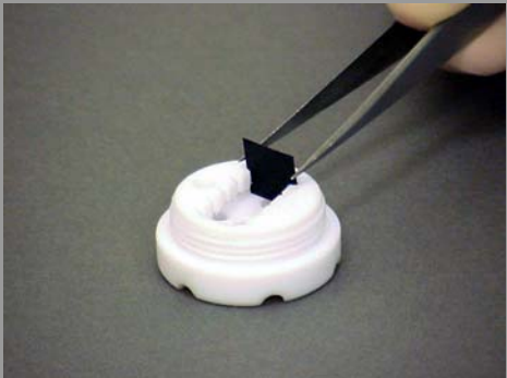
Load 10mm square chip into each slot of the bottom part. You may load up to 5 die
